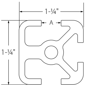
SL-SQPROF3W (270° 3-slot)
