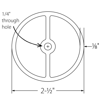
SL-2.5BAR (2.5" extrusion)
