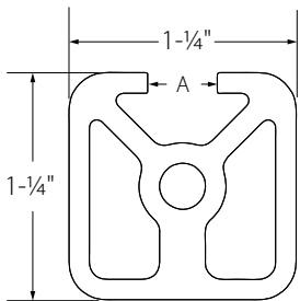
SL-SQPROF (Single-slot)
