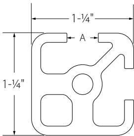
SL-SQPROF90 (90° 2-slot)
